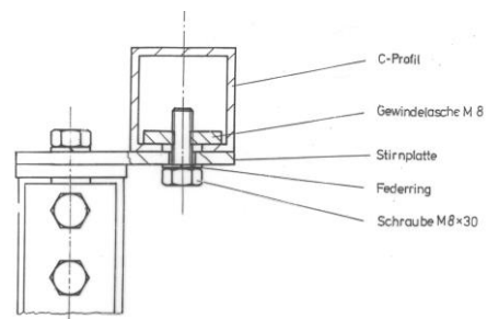
Side view Plate with 2 holes
