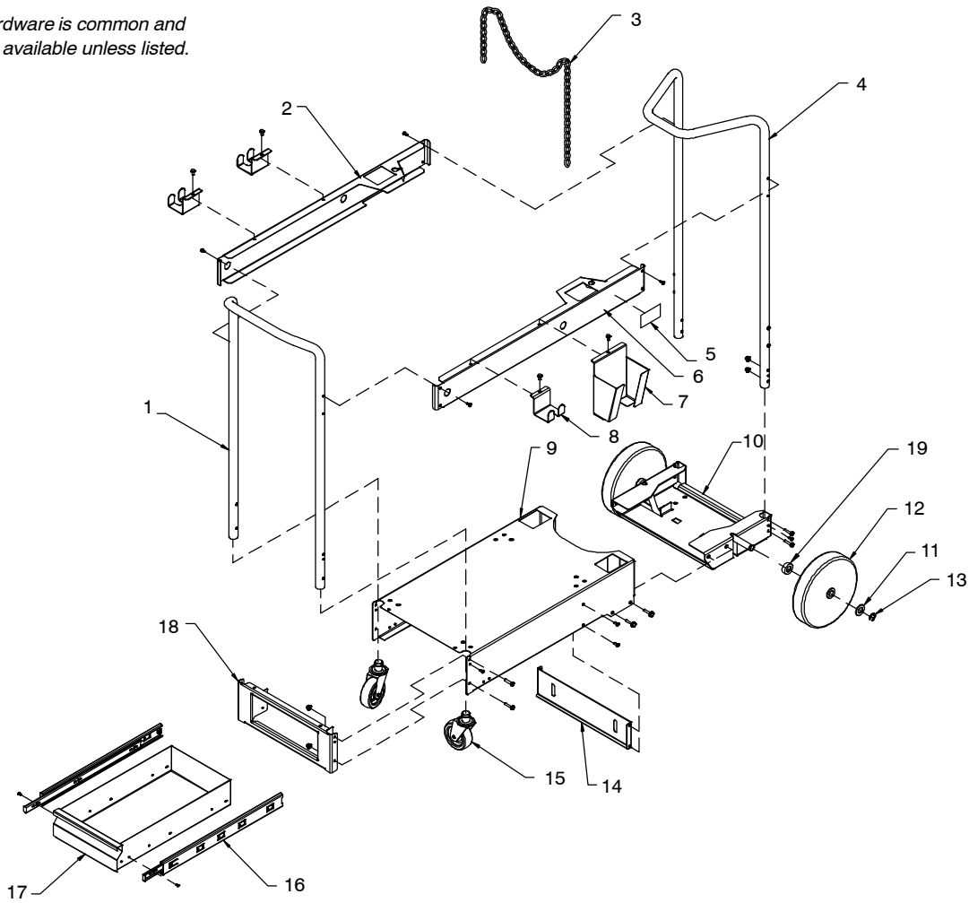
Figure 1-1. Complete Assembly
